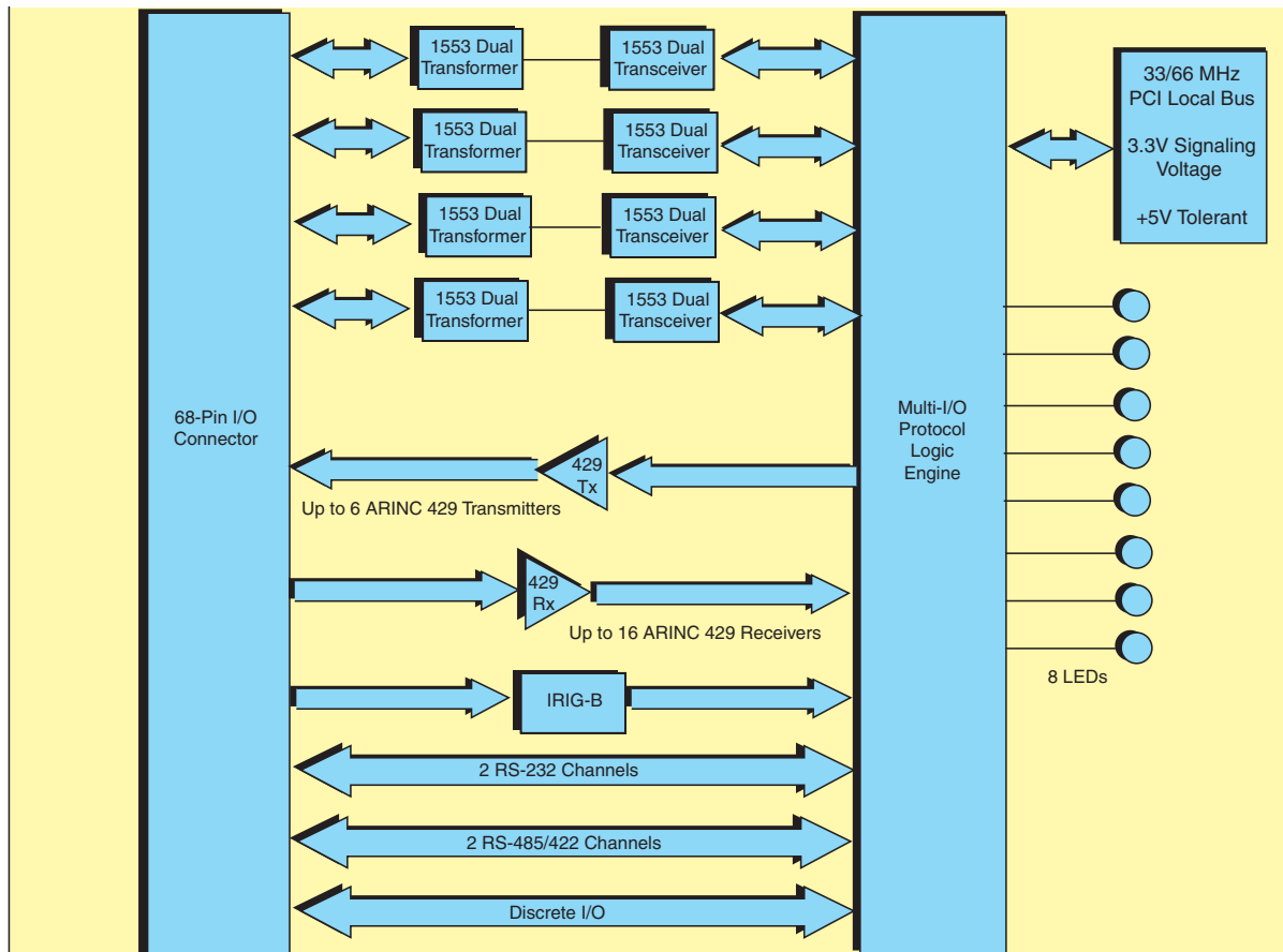
Figure 1. BU-65590F/M Block Diagram
