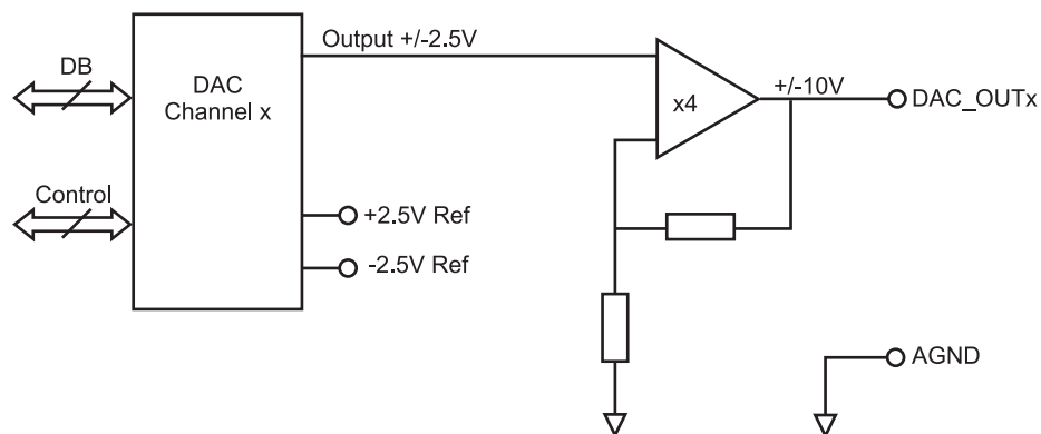
Figure 5-4 : Output Wiring
