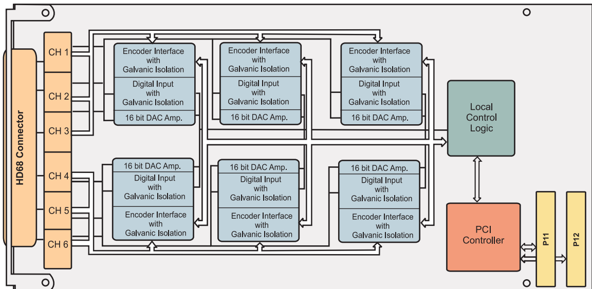
Figure 1-1 : Block Diagram
