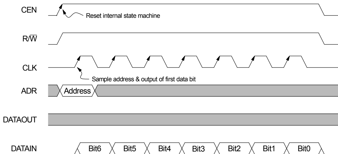
Figure 5-3 : CPLD-Bus Read
