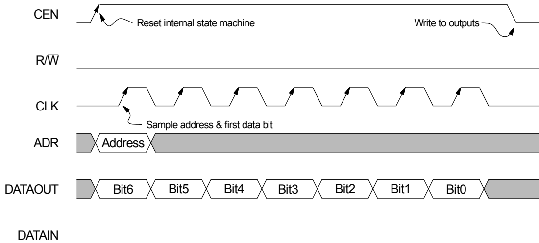
Figure 5-2 : CPLD-Bus Write
